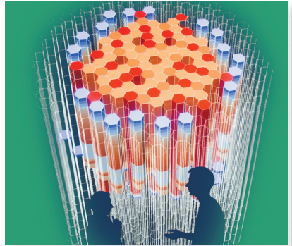
Neutronics and thermal-hydraulics Coupling for SMR simulation
