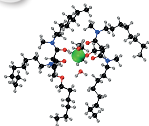
Actinide complex solvated by extraction molecule
